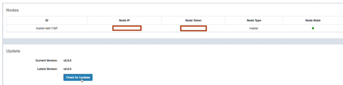
FIGURE 1 Updating software
